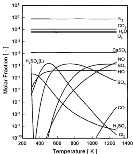
Fig. 2. The molar fraction of major gaseous pollutants as a function of temperature under the conditions of 0.1% of chlorine in the waste and 90% \text{SO}_2 -removal.
